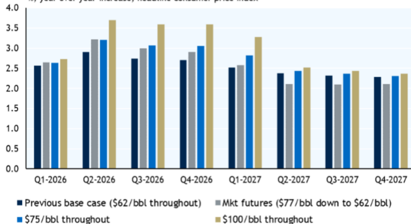
U.S. headline CPI projections by oil price scenarios
